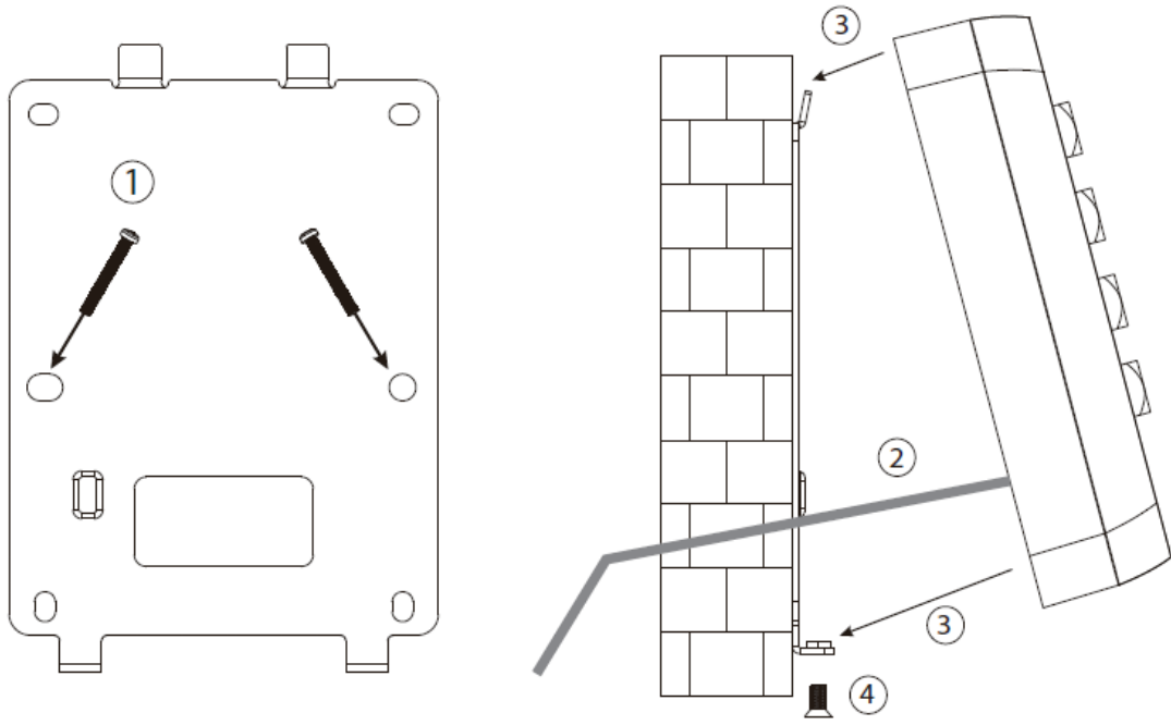
Figure 2-1 Drill holes (mm[inch])
