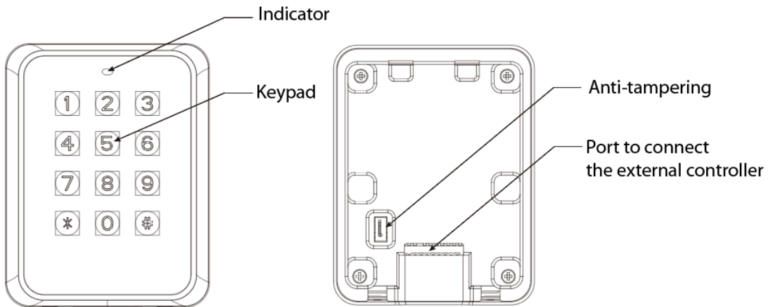
Figure 1-1 Appearance (model M)
