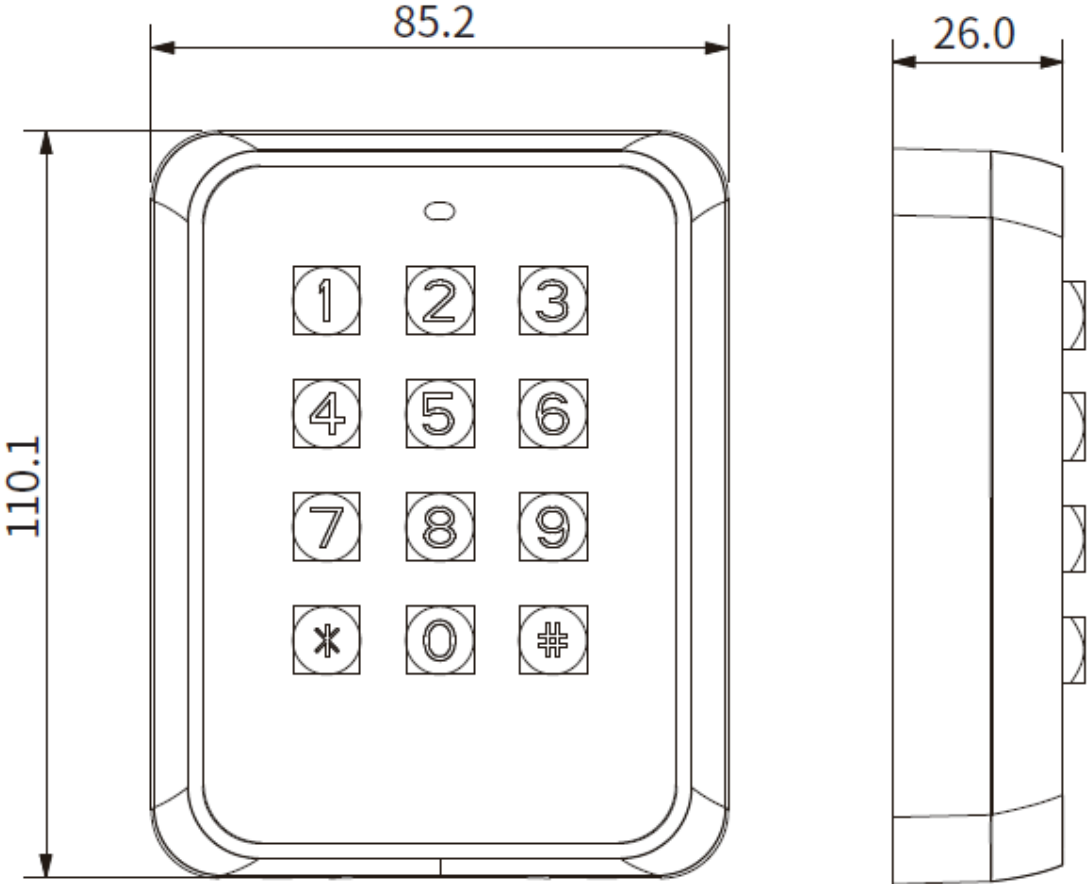
Figure 1-2 Dimensions (Model M) (mm [inch])
